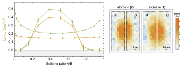
FIG. 2. Entanglement quantification in split spin-squeezed BECs. Lower bounds on the BSA and the GR, as obtained from Eq. (15) according to Lemma 3. Measurements are taken from a spin-squeezed BEC of N = 590 atoms. The dotted lines show the maximum amount of entanglement that could be explained by detection cross talk [34]. On the right, we show single-shot absorption images of the atomic densities for the two internal degrees of freedom, with an example of regions A and B used to define the collective spins J^A and J^B .
