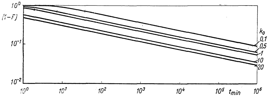
Fig. 5. Relationship \log(1 - F) vs. \log t for 100 components ( n = 100 , \Omega/RT = 1 , and different values of k_0 )
