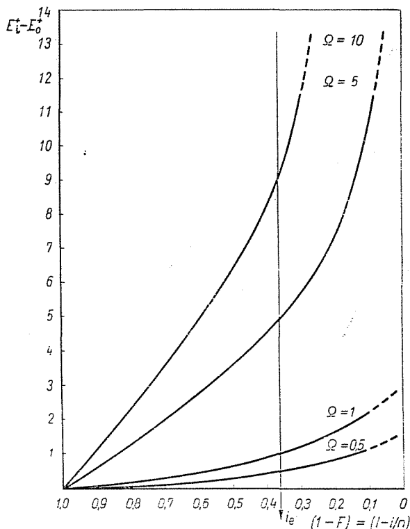
Fig. 1. Relationship E_i^+ - E_0^+ vs. (1 - F) calculated according to Eq. (2) for \Omega = 10, 5, 1 and 0.5
