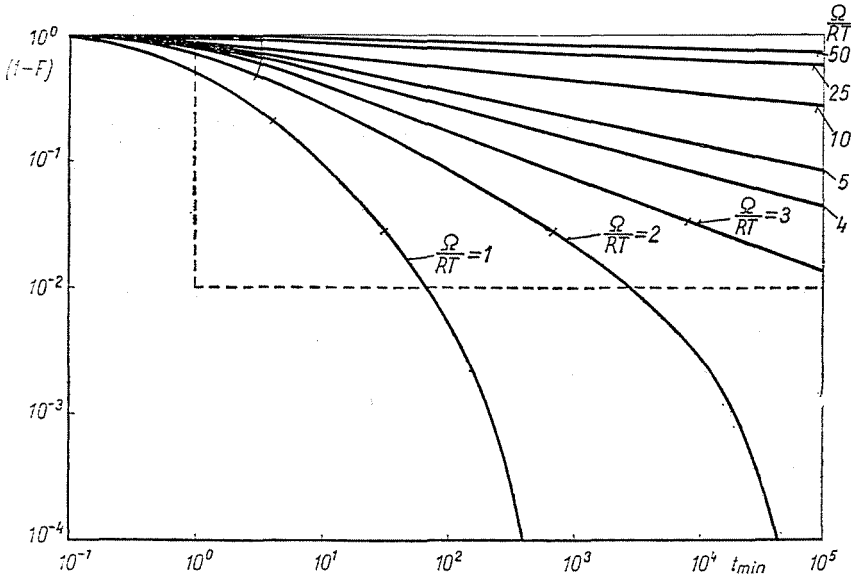
Fig. 4. Relationship \log(1 - F) vs. \log t for 100 components ( n = 100 ), k_0 = 1 , and different values of \Omega/RT
