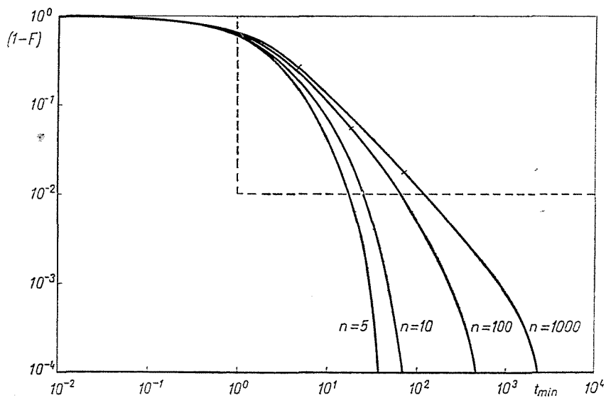
Fig. 3. Relationship \log(1-F) vs. \log t for k_0 = 1 , \Omega/RT = 1 and different values of n
