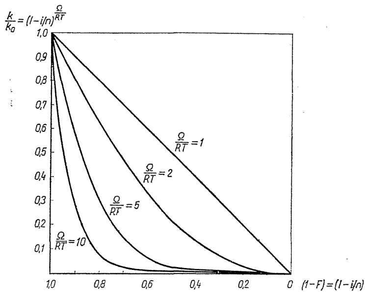
Fig. 2. Relationship k_i vs. (1-F) calculated according to Eq. (5)
